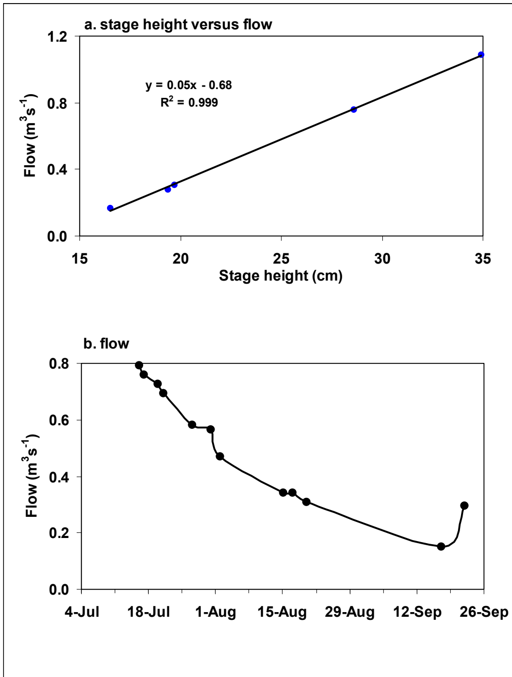
Figure 3. Streamflow gauge calibration (a.) and flow (b.) of Marys River at Cloud Run Farm (site 4 in Figure 2), Oregon, summer 1998.
